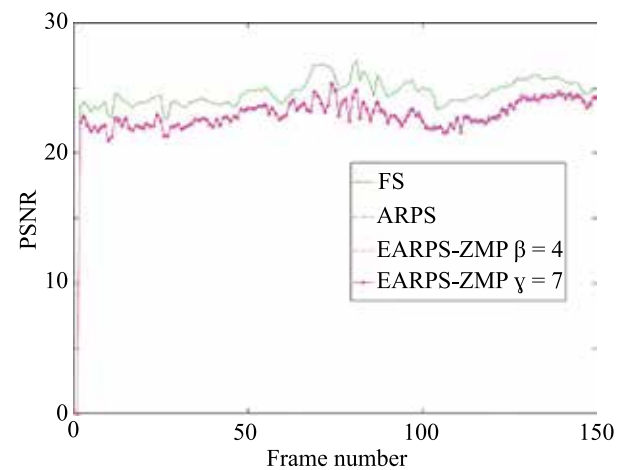
Fig. 7. PSNR Comparison of FS, ARPS, and EARPS algorithms on “bus” video sequence
