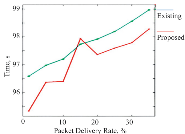
Fig. 7. Performance Analysis of Packet Delivery Ratio of Multiple Mobile Sink
