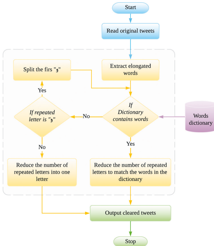
Fig. 6. Elongated words spelling correction process
