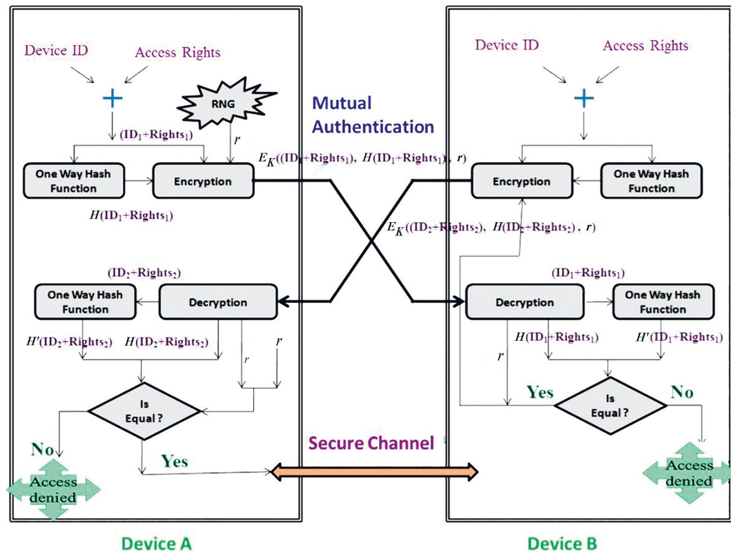
Fig. 2. The Proposed Protocol Architecture
