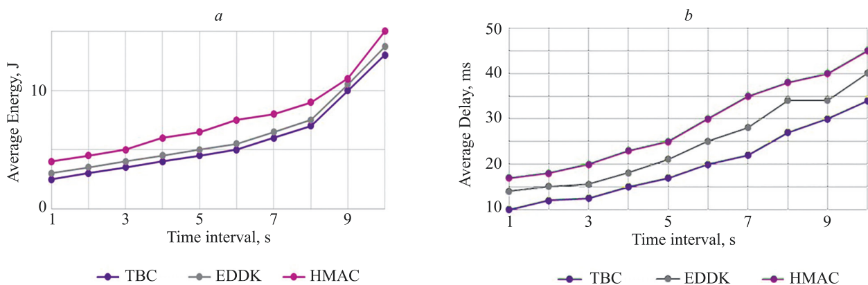
Fig. 3. Performance analysis of the proposed work. Energy Comparative Analyzes: power consumption ( a ), average delay ( b ) and throughput ( c ) of EDDK, HMAC and TBC. Average power consumption by malicious nodes ( d ), analysis of average latency by malicious nodes ( e )
