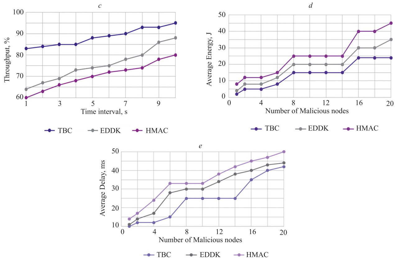
Fig. 3. Performance analysis of the proposed work. Energy Comparative Analyzes: power consumption (a), average delay (b) and throughput (c) of EDDK, HMAC and TBC. Average power consumption by malicious nodes (d), analysis of average latency by malicious nodes (e)
