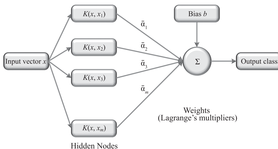
Fig. 3. Structure of SVM, where K(u, v) is a kernel function satisfying Mercer's condition; x is a point of hyperplane; x_i are support vectors; \bar{\alpha}_i are Lagrange's multipliers; m is SVM hyperplane dimension; and b is a bias
