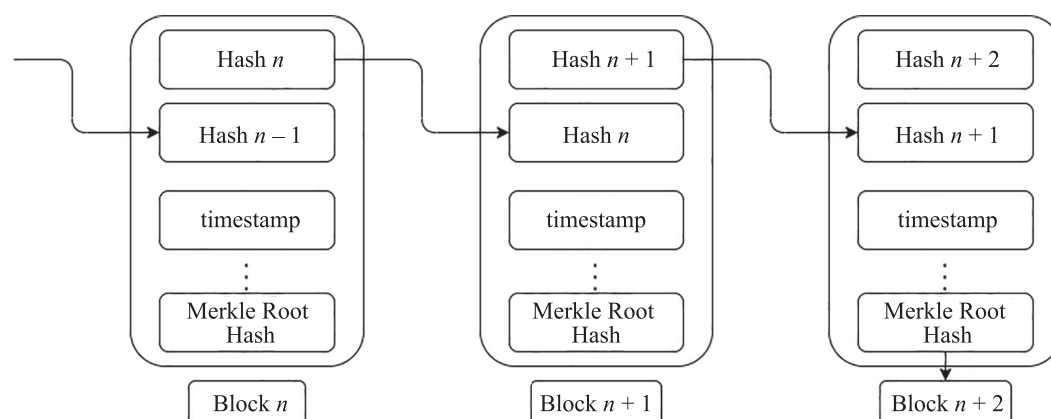
Fig. 1. Blockchain basic structure
