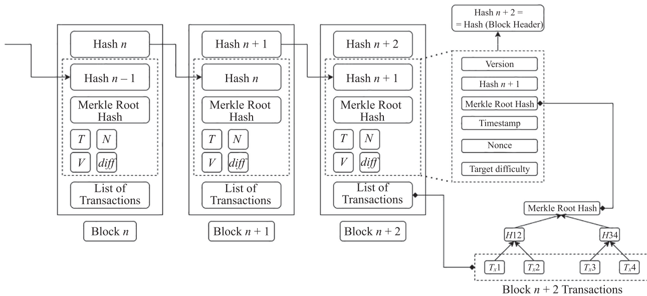
Fig. 2. Bitcoin's detailed structure
