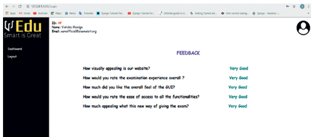
Fig. 6. Feedback webpage
