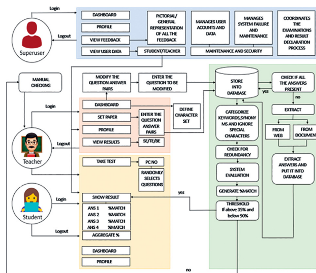
Fig. 1. Activity Diagram for Web Based Application System for Revolutionary Assessment and Instant Evaluation
