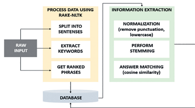
Fig. 2. Natural language processing modules for revolutionary assessment and instant evaluation
