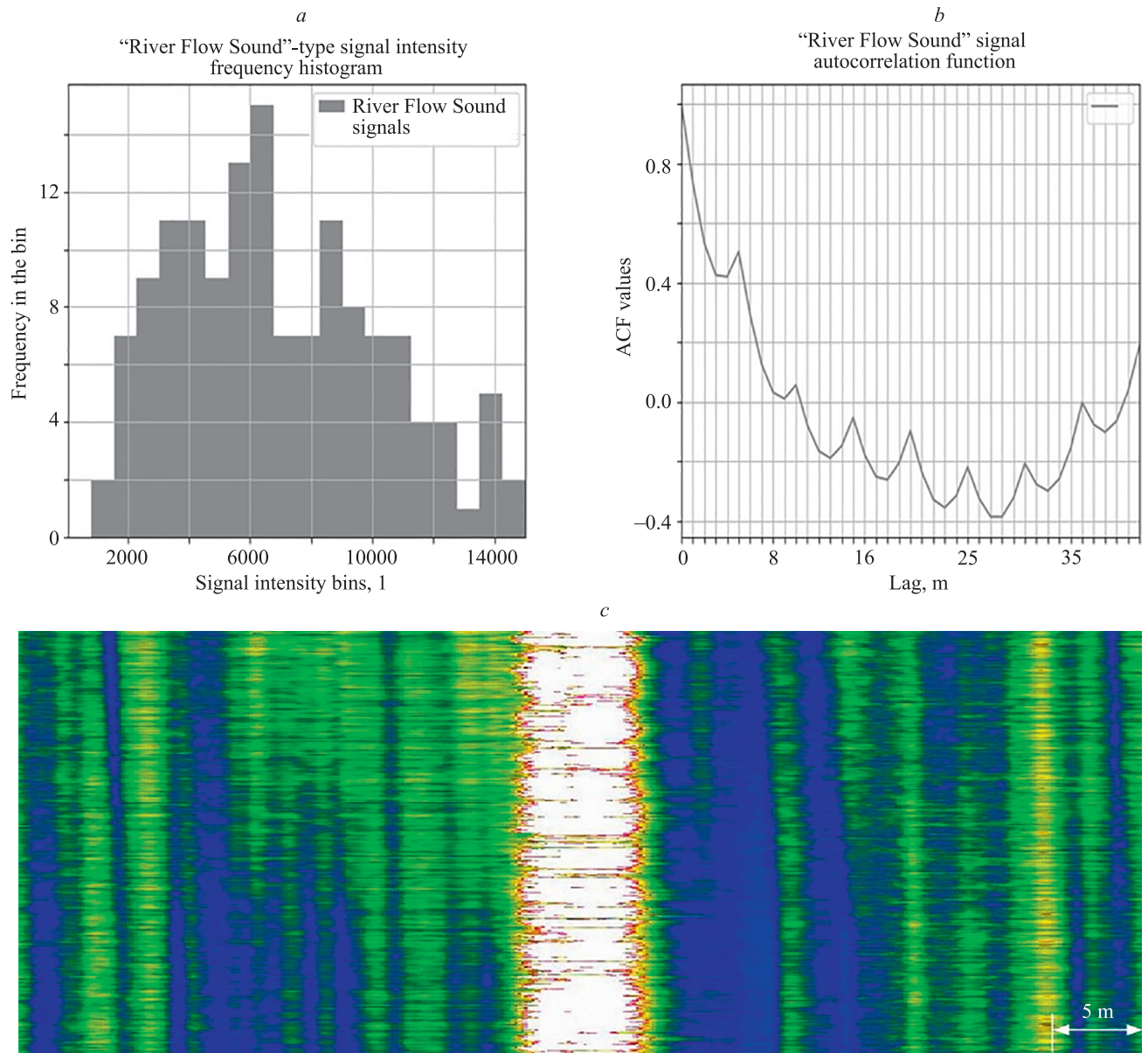
Fig. 5. Typical histogram (a), autocorrelation function (b), and waterfall diagram (c) for class 0, “River Flow Sound”
