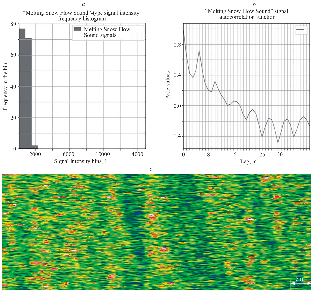
Fig. 6. Typical histogram (a), autocorrelation function (b), and waterfall diagram (c) for class 1, "Melting Snow Flow Sound"
