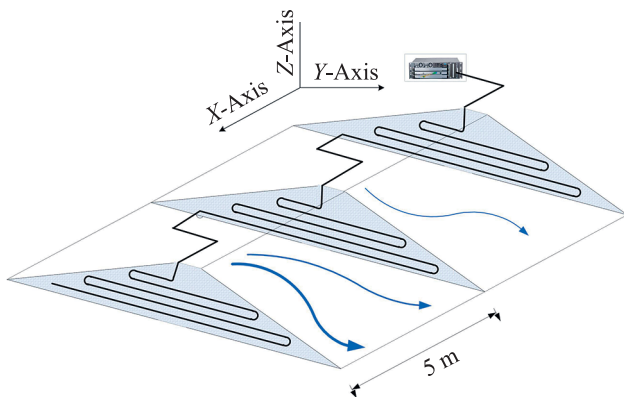
Fig. 9. Installation of a fiber-optic sensor in a tailings dam body
