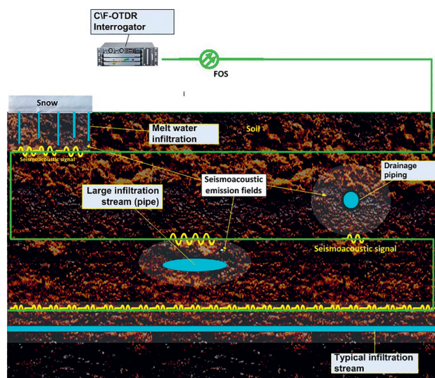
Fig. 2. Installation scheme of DAS monitoring system in the tailings dam body.
