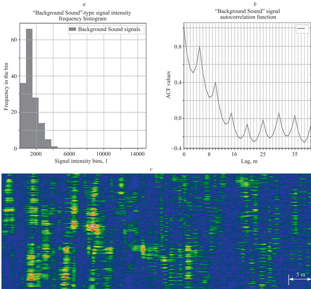
Fig. 8. Typical histogram (a), autocorrelation function (b), and waterfall diagram (c) for class 3, "Background sound"
