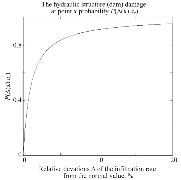
Fig. 4. Function P(\Delta(\mathbf{x})|a_x)
