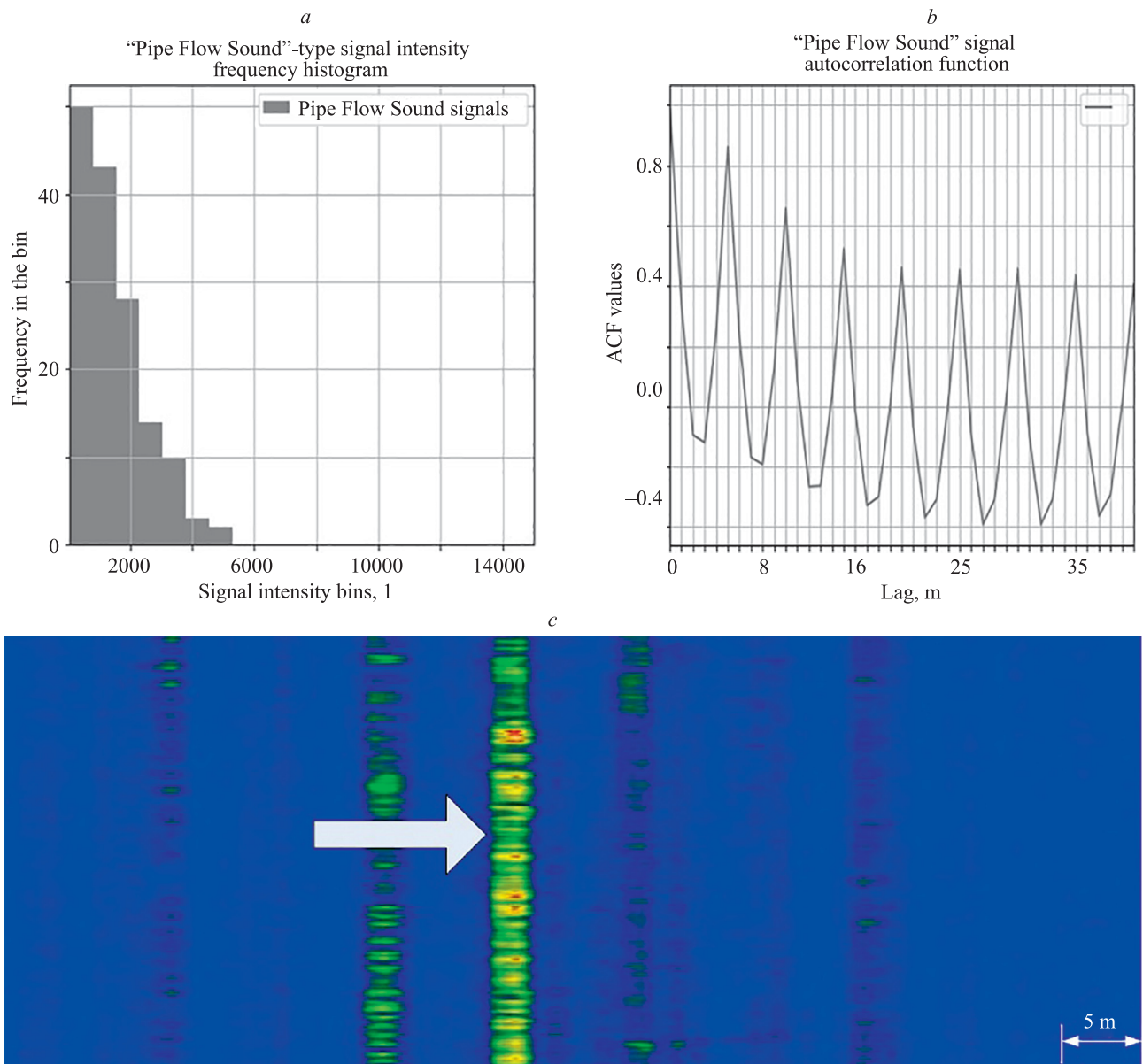
Fig. 7. Typical histogram (a), autocorrelation function (b), and waterfall diagram (c) for class 2, "Pipe Flow Sound"
