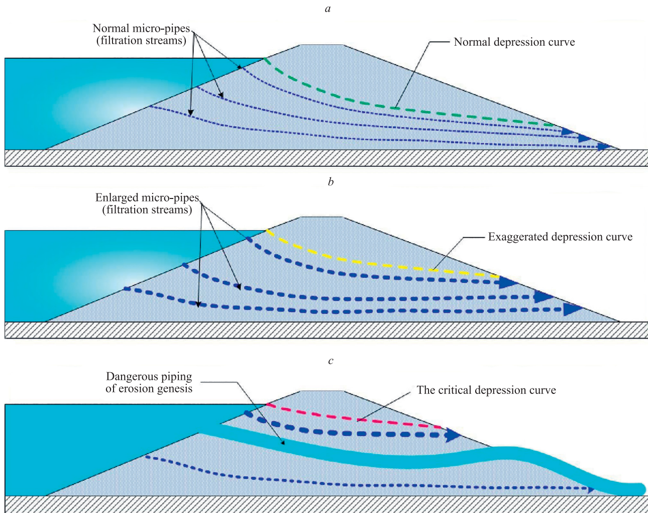
Fig. 1. Stages of infiltration process progression inside the dam body: normal situation (a); infiltration increasing, pre-critical situation (b); maximum infiltration process development, critical situation (c)
