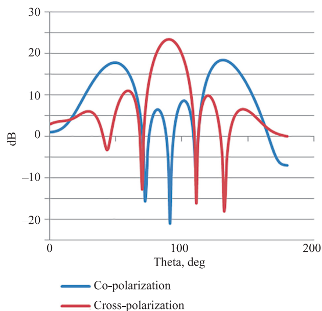
Fig. 17. Hardware model experimental result for co-gain &amp; cross-polarization gain
