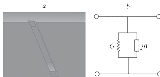
Fig. 2. Inclined slots in narrow wall with semicircular cutting: inclined slot (a); admittance of the slot where G is the conductance and jB is the susceptance (b)
