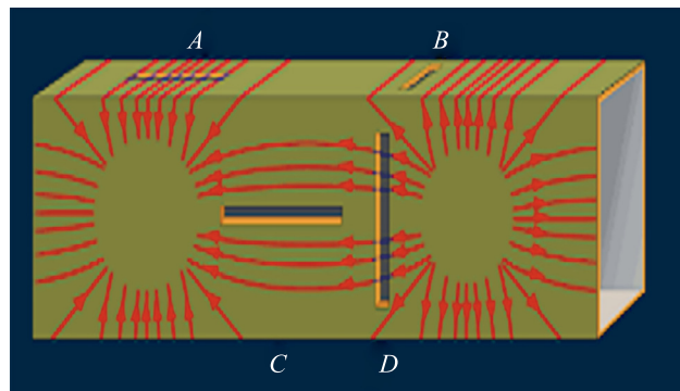
Fig. 4. Typical slots over rectangular waveguide:
