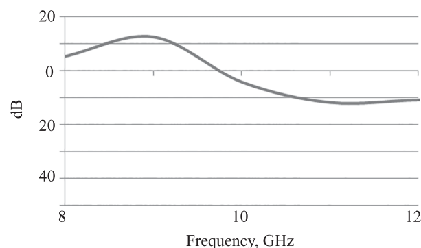
Fig. 11. HFSS result for ten inclined slots in narrow wall without semicircular cutting
