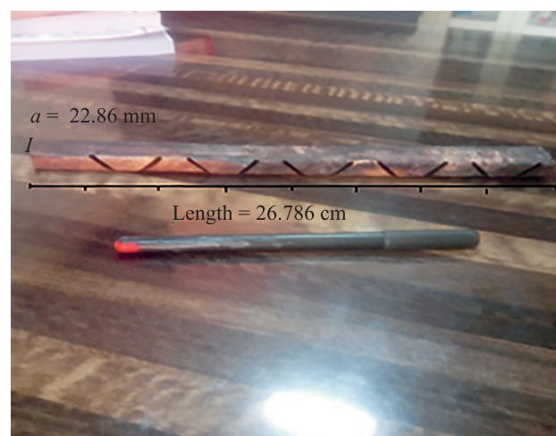
Fig. 5. Designed waveguide with 10 inclined slot
