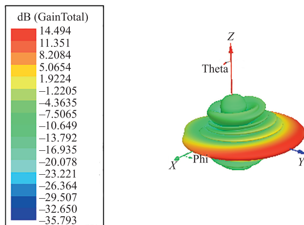
Fig. 16. 3D radiation pattern in HFSS
