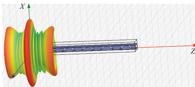
Fig. 9. Waveguide designed for ten slots
