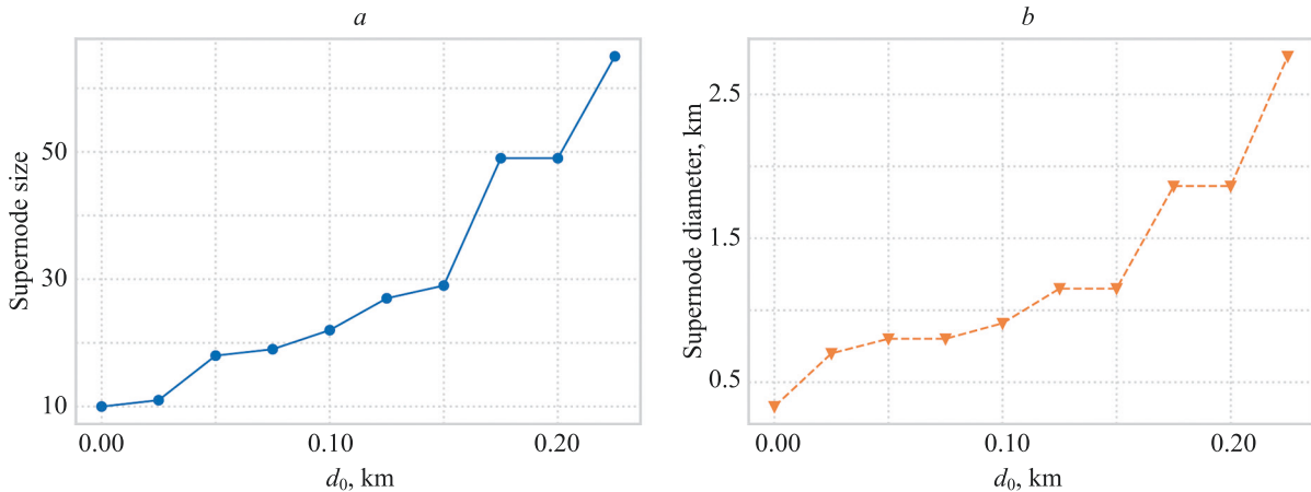
Fig. 6. Maximal supernode size (a) and diameter (b) for different values of d_0 . Even for relatively small values ( d_0 > 0.15 ) these characteristics grow quite rapidly resulting in some supernodes having diameter as large as 2 km and more
