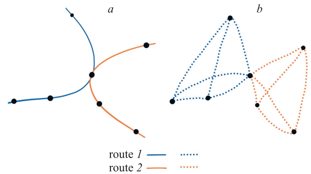
Fig. 1. Difference between L-space (a) and P-space (b)
