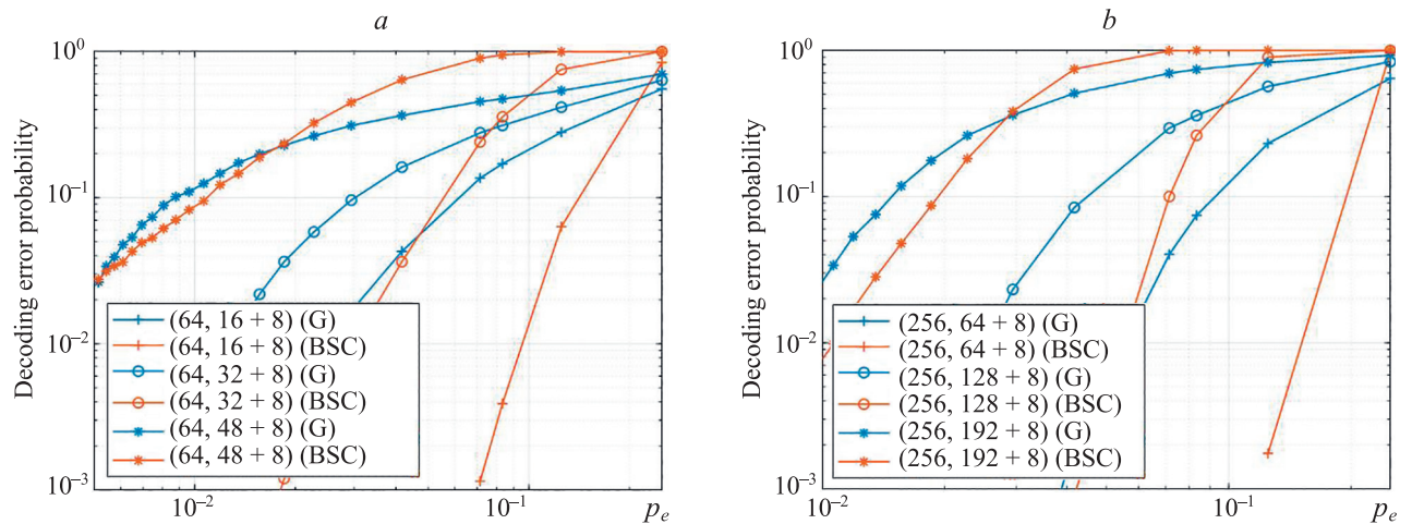
Fig. 7. Decoding error probability for: n = 64 (a); n = 256 (b)
