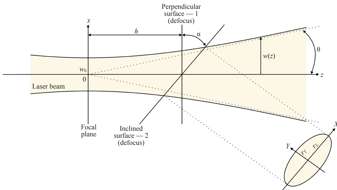
Fig. 4. Schematic of laser beam interaction on material surface; r_T is minor axis of ellipse; r_L is major axis of ellipse
