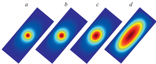
Fig. 7. Surface heat treatment of positive laser beam spot defocus on inclined or uneven material surface with variable: \alpha = 0 , h = 0 mm (a); \alpha = 0.436 rad, h = 25 mm (b); \alpha = 0.873 rad, h = 50 mm (c); \alpha = 1.309 rad, h = 75 mm (d)
